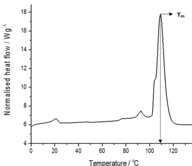
Figure 6. A DSC thermogram of G4LZI3. The protein is shown to have a transition temperature of approximately 110°C.
