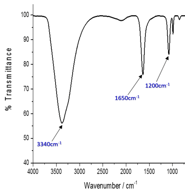
Figure 5. FTIR spectrum of G4LZI3. Three prominent peaks are shown, indicating the secondary structure element and functional groups present in the protein.
