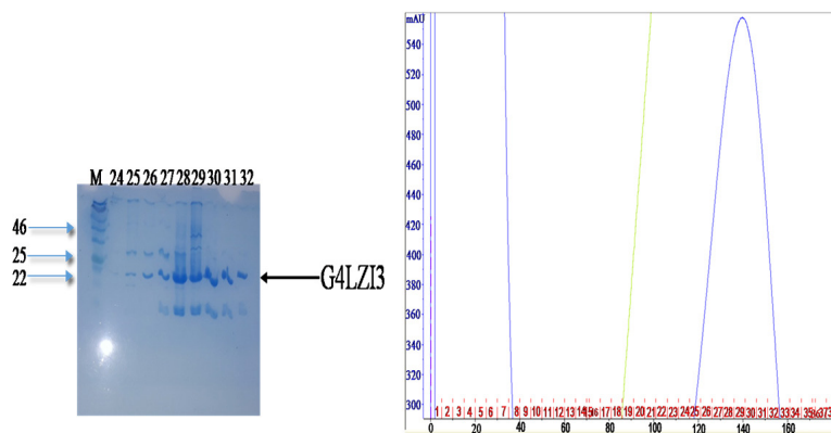
Figure 3. Affinity purification chromatogram and SDS PAGE gel. The peak was observed at a high imidazole concentration, indicating elution of G4LZI3 protein. The SDS PAGE gel on the left side shows fractions from the peak. The tight bands at approximately 20.3 kDa indicate partially successful purification of the protein. The bands observed at around 20 kDa are indicative of either protein degradation or the presence of a contaminating protein, hence a second purification step was necessary.
