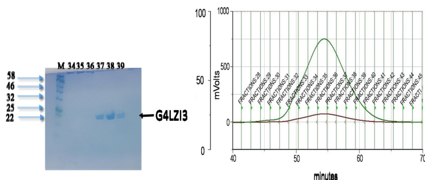
Figure 4. SEC chromatogram and SDS PAGE gel. Chromatogram showing separation of G4LZI3 from high molecular weight impurities present in the affinity-purified sample. SDS PAGE gel on left shows G4LZI3 protein to be running at the expected size of 20.3 kDa from fractions 34, 35, 36, 37, 38 and 39.
