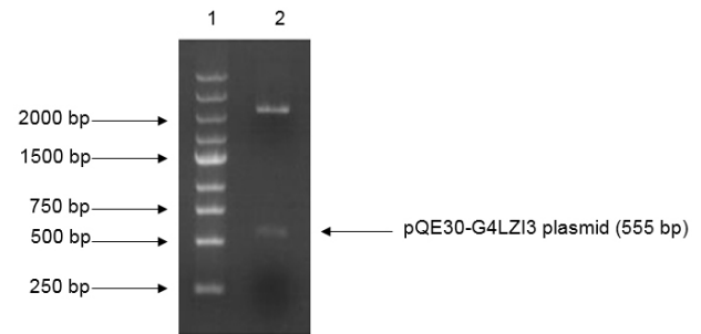
Figure 1. Restriction digest gel for confirmation of G4LZI3 insert fragment. Lane 1 is the DNA marker, lane 2 is the plasmid digested by BamHI and HindIII.
