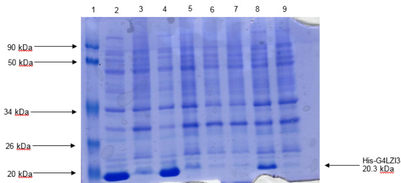
Figure 2. Expression screen of transformed colonies from pQE30-G4LZI3 for protein expression. Lane 1 is the protein molecular weight marker, lanes 2, 4, 6 and 8 indicate the total bacterial cell lysates after induction of protein expression with addition of 0.5 mM IPTG, while lanes 3, 5, 7 and 9 indicate the corresponding total bacterial cell lysates of the un-induced cultures. The induced lanes (2, 4 and 8) show bands of approximately 20.3 kDa, corresponding to the His-G4LZI3 fusion protein.
