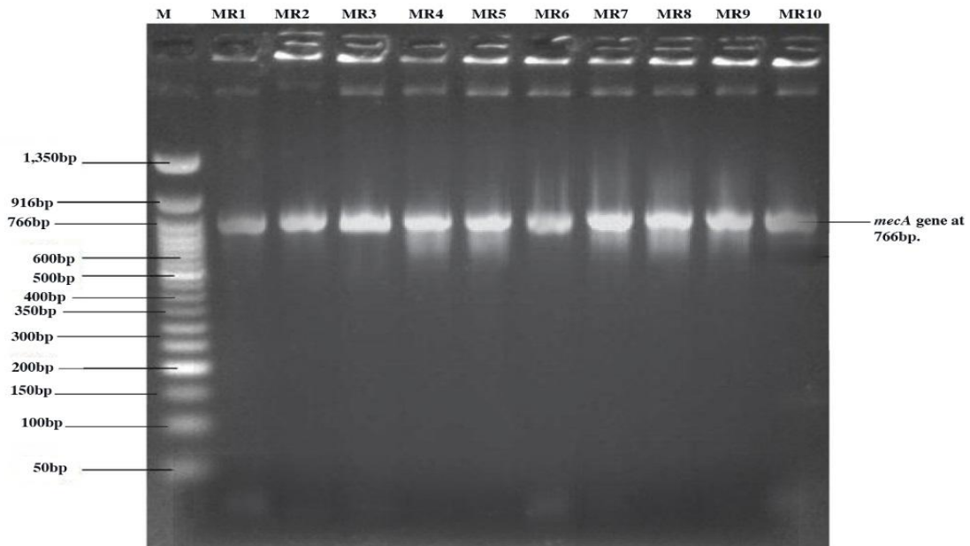
Fig. 3. Amplification of MRSA mecA gene
