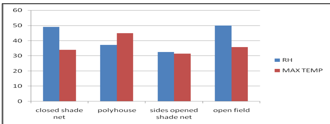
Fig. 3. Temperature and Relative humidity recorded in different protected structures during February, 2022
