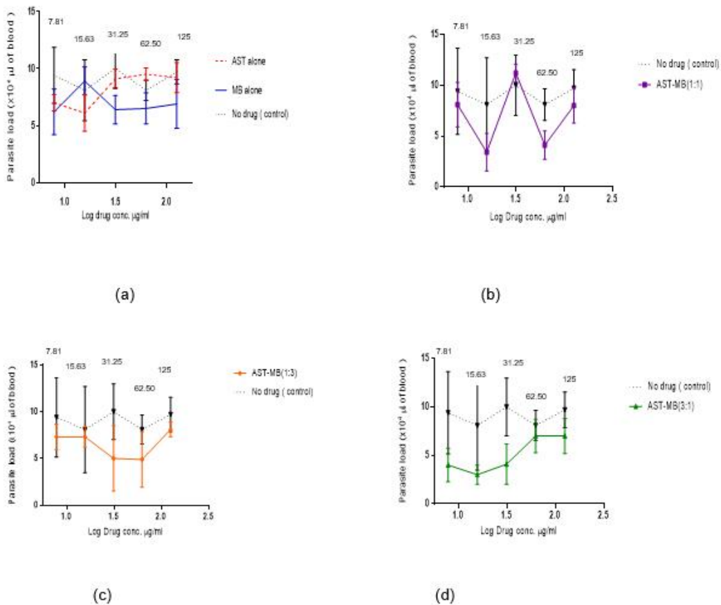
Fig. 1. Parasitemia of drugs and the control against Plasmodium falciparum 3D7 (a) astemizole alone and methylene blue alone, (b) astemizole-methylene blue drug combination (1:1), (c) astemizole-methylene blue drug combination (1:3), (d) astemizole-methylene blue drug combination (3:1)
