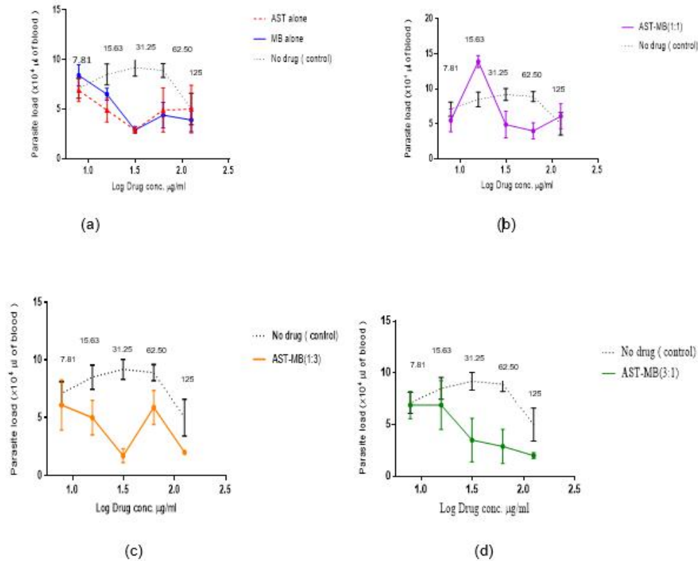
Fig. 2. Parasitemia of drugs and the control against Plasmodium falciparum W2 (a) astemizole alone and methylene blue alone, (b) astemizole-methylene blue drug combination (1:1), (c) astemizole-methylene blue drug combination (1:3), (d) astemizole-methylene blue drug combination (3:1)
