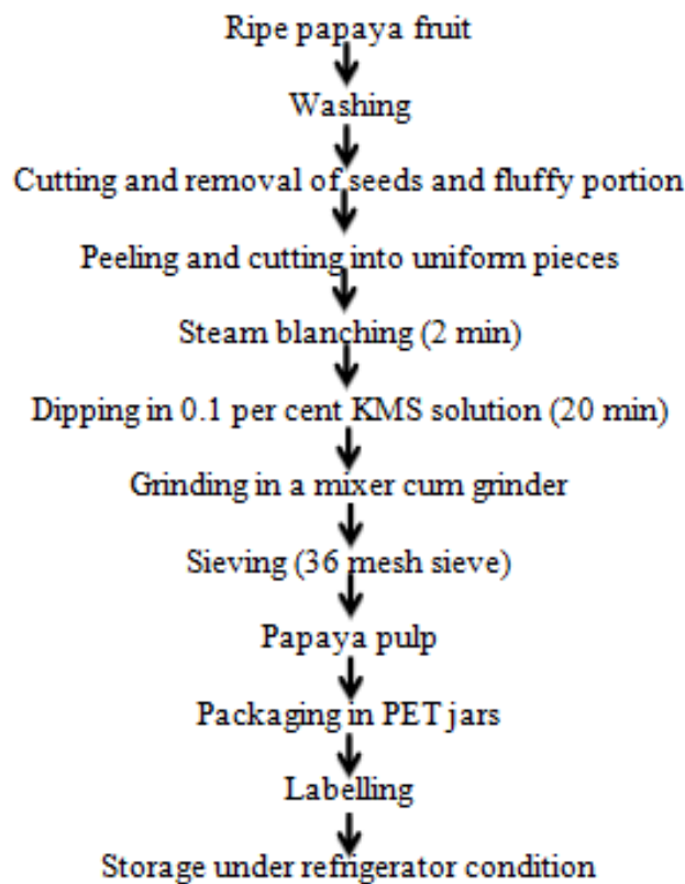
Fig. 1. Unit operations for preparation of papaya pulp
