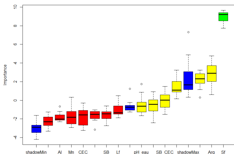
Fig. 11. Boxplot of importance of feature selection influencing total iron at the summit topographic position, using the Boruta algorithm
