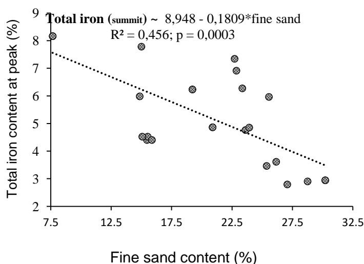
Fig. 12. Linear relationship between total iron and fine sand at 0-20 cm under rubber cultivation
