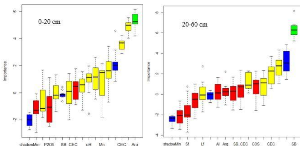
Fig. 6. Boxplot of importance of selection of characteristics under rice cultivation at 0-20 cm and 20-60 cm, using the Boruta algorithm
