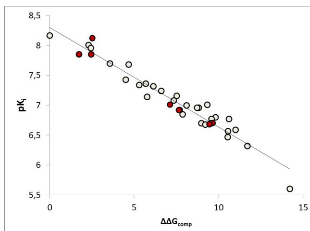
Fig. 3. Plot for relative complexation Gibbs free energies of the PPO-CQBx complex formation \Delta\Delta G_{\text{com}} [kcal.mol -1 ] of the training set [15]. The validation set data points are shown in red color
