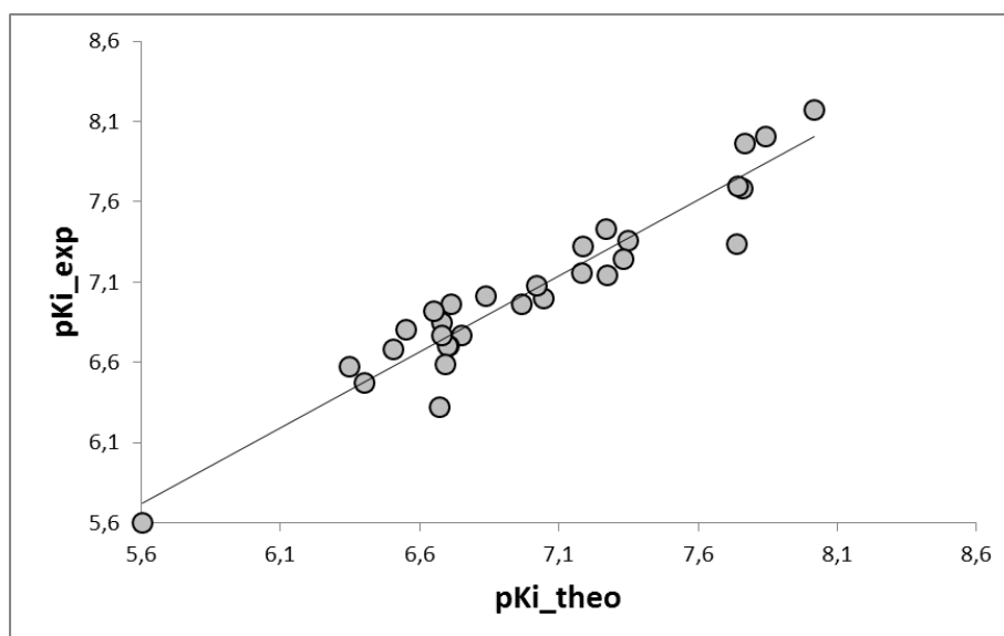
Fig. 4. (A) Distances between centers, (B) angles between centers of pharmacophoric features (C) features, (D) mapping of pharmacophore of ligand with the most partial agonist 17i. Feature legend: HYDA = Hydrophobic Aliphatic (blue), HBA = Hydrogen bond Acceptor (green). (E) Correlation plot of experimental vs. predicted activation activity
