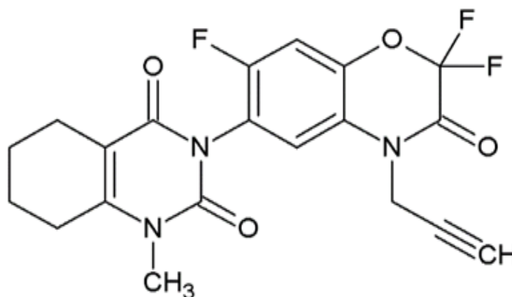
Fig. 1. Chemical structure of herbicidal agents: Cycloalka[d]quinazoline-2,4dione–Benzoxazinones core (17i)
