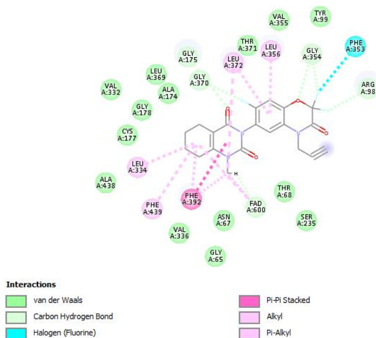
Fig. 2. PPO-17i – ligand interactions at active site depicted in 2D for the most active CQB
