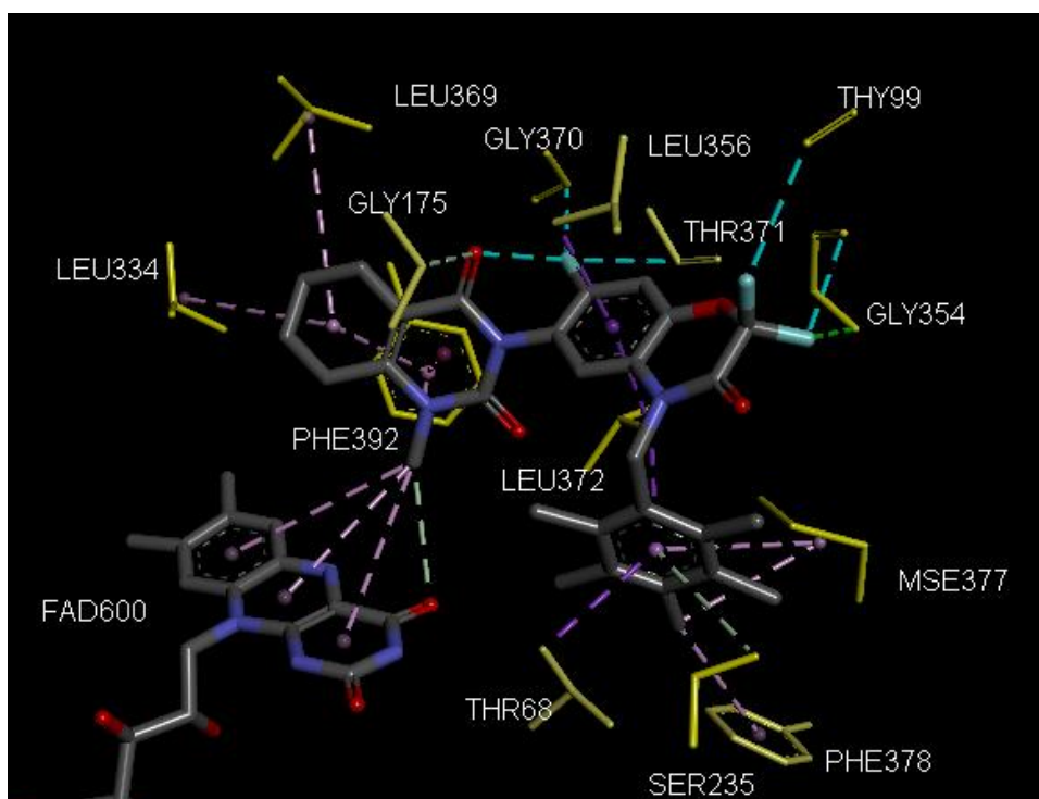
Fig. 5. (A) 2D schematic interaction diagram of the most potent inhibitor CQB22 at the active site of PPO and (B) 3D schematic interaction
