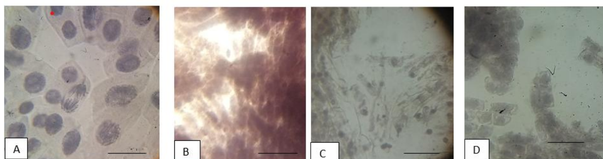
Fig. 2. Treatment effects on onion cells: A is Control with dividing cells (bar= 10μ); B is 36hrs treatment with charred cells (bar=25μ); C is 72hrs treatment with broken up cells (bar= 25μ); D is 120hrs with intact but non-dividing cells (bar=25μ)
