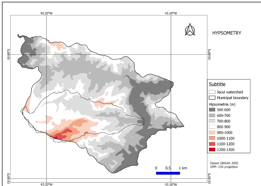
Fig. 2. Hypsometric map Source: Author (2023)
