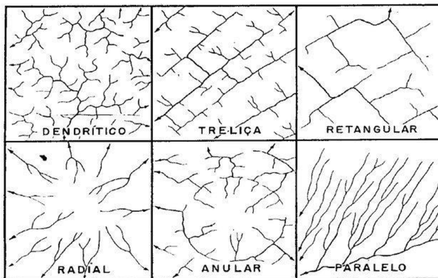
Fig. 3. Drainage patterns Source: Fryis and Brierley (2013)
