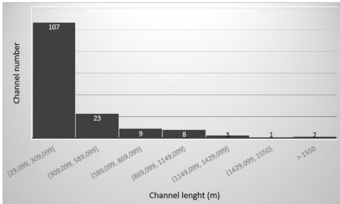
Fig. 4. Length of drainage channels in the Jacuí River watershed
