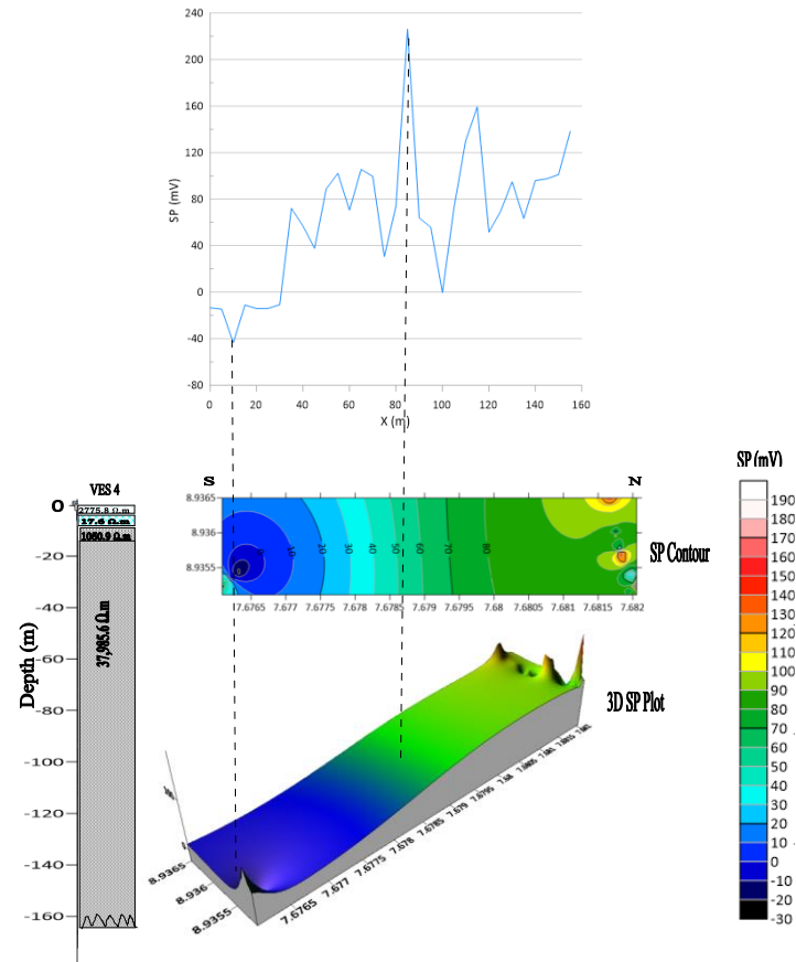
Fig. 22. Cross-section correlating the VES transverse, Self-Potential in (mV) signal, SP contours and 3-D SP plot along Profile 4
