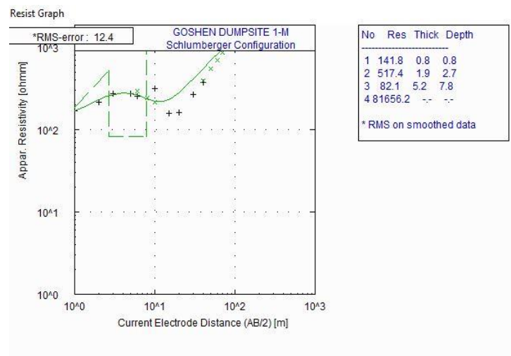
Fig. 13. Results of computer modeled curve for VES 12
