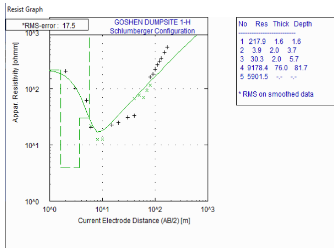
Fig. 9. Results of computer modeled curve for VES 8
