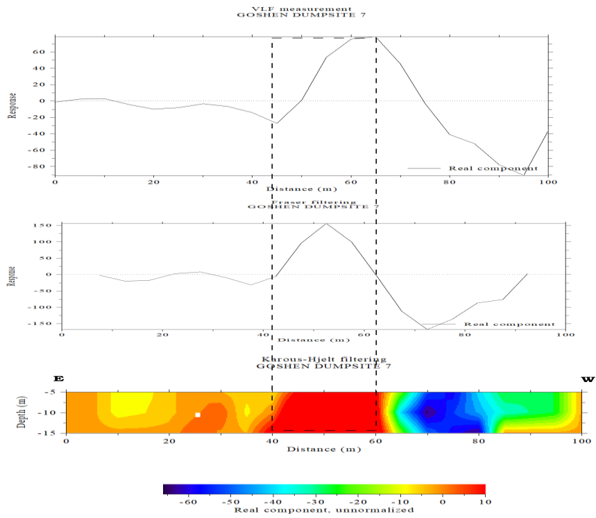
Fig. 35. Cross-section of Fraser Filtered, measured VLF and K-H pseudo section along Transverse 7
