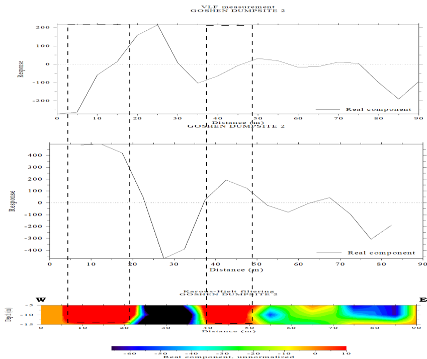
Fig. 30. Cross-section of Fraser Filtered, measured VLF and K-H pseudo section along Transverse 2
