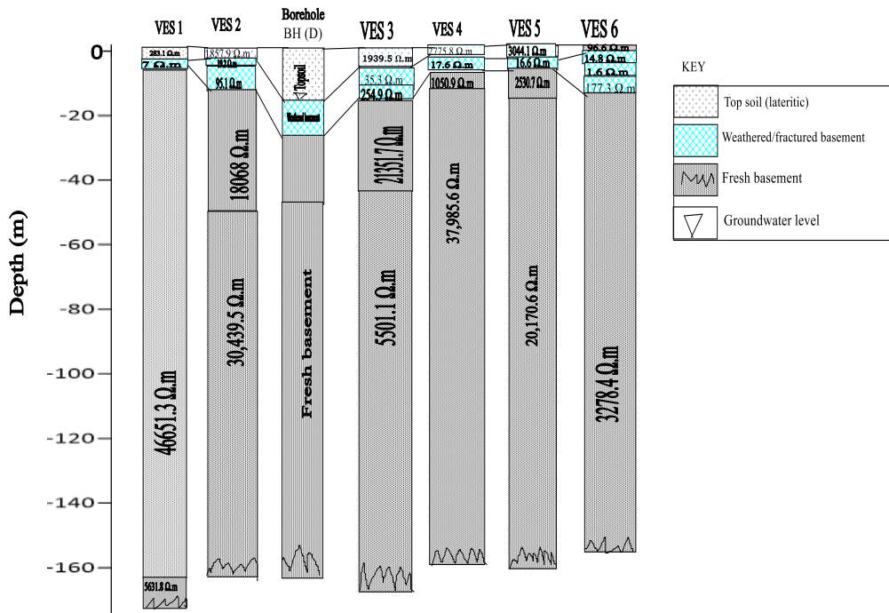
Fig. 17. Correlation of resistivity sounding (VES) results with borehole lithological logs in the study area
