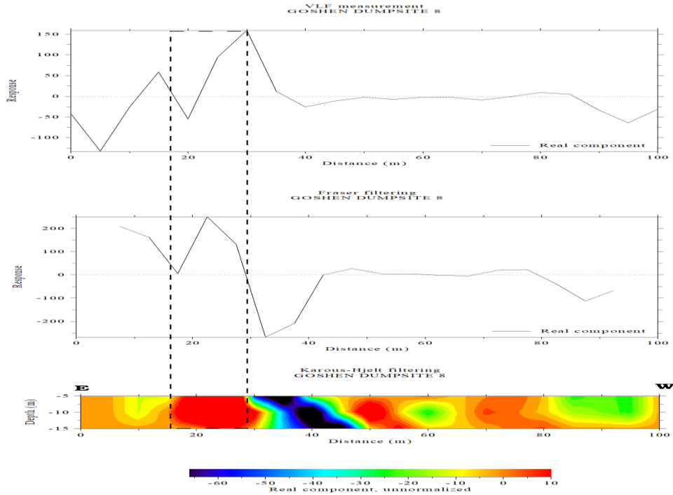
Fig. 36. Cross-section of Fraser Filtered, measured VLF and K-H pseudo section along Transverse 8
