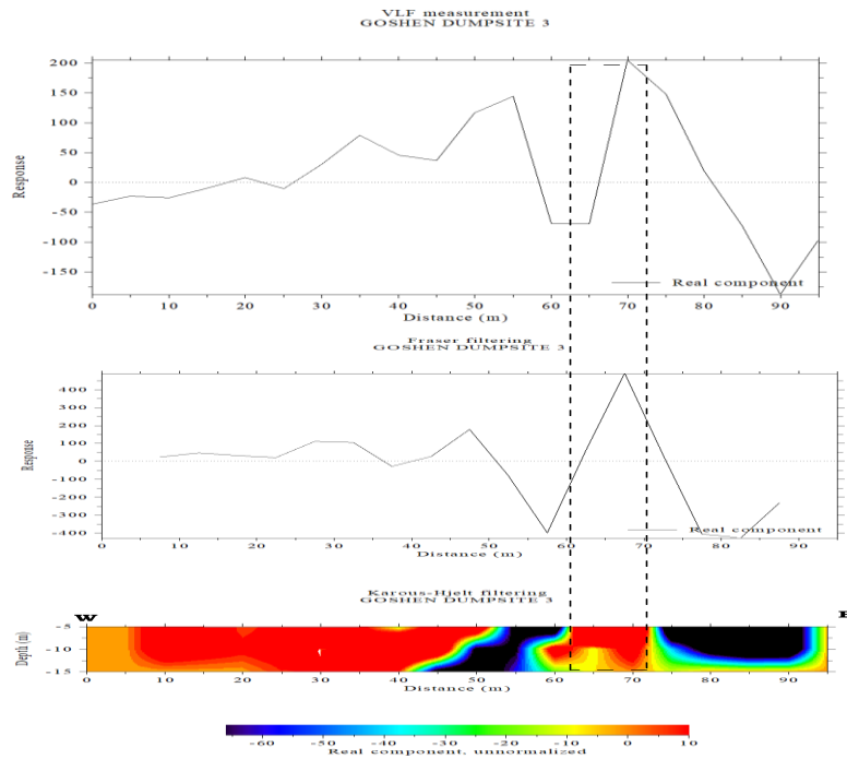
Fig. 31. Cross-section of Fraser Filtered, measured VLF and K-H pseudo section along Transverse 3
