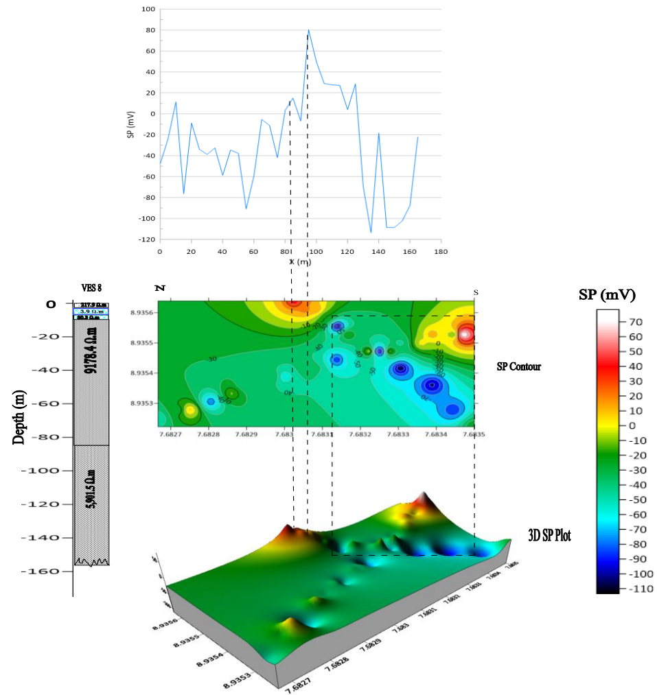
Fig. 26. Cross-section correlating the VES transverse, Self-Potential in (mV) signal, SP contours and 3-D SP plot along Profile 8
