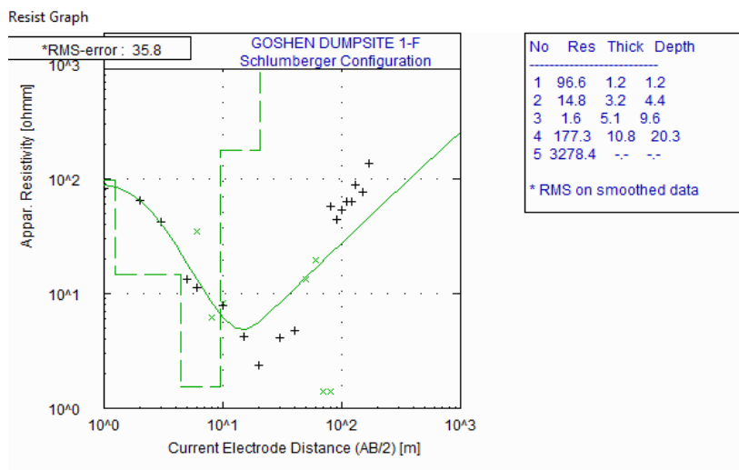
Fig. 7. Results of computer modeled curve for VES 6
