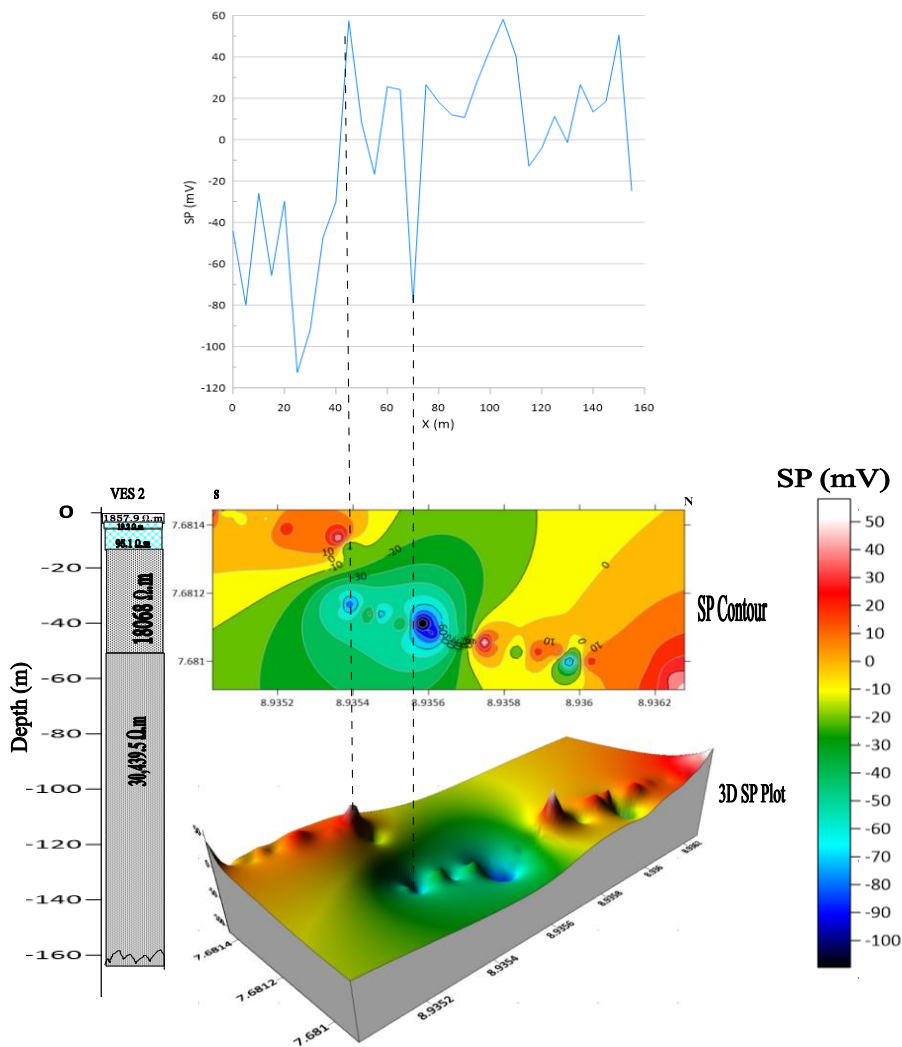
Fig. 20. Cross-section correlating the VES transverse, Self-Potential in (mV) signal, SP contours and 3-D SP plot along Profile 2
