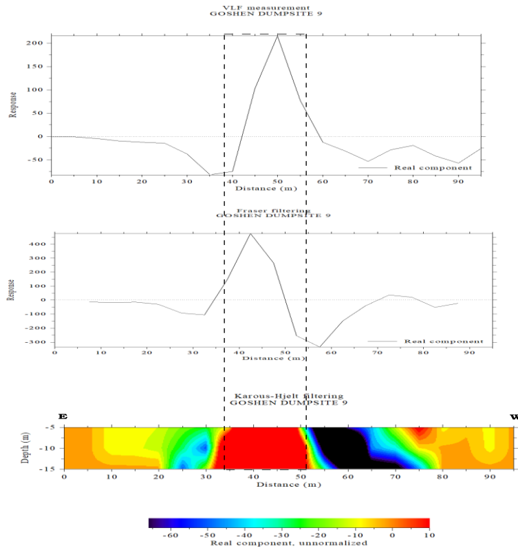
Fig. 37. Cross-section of Fraser Filtered, measured VLF and K-H pseudo section along Transverse 9
