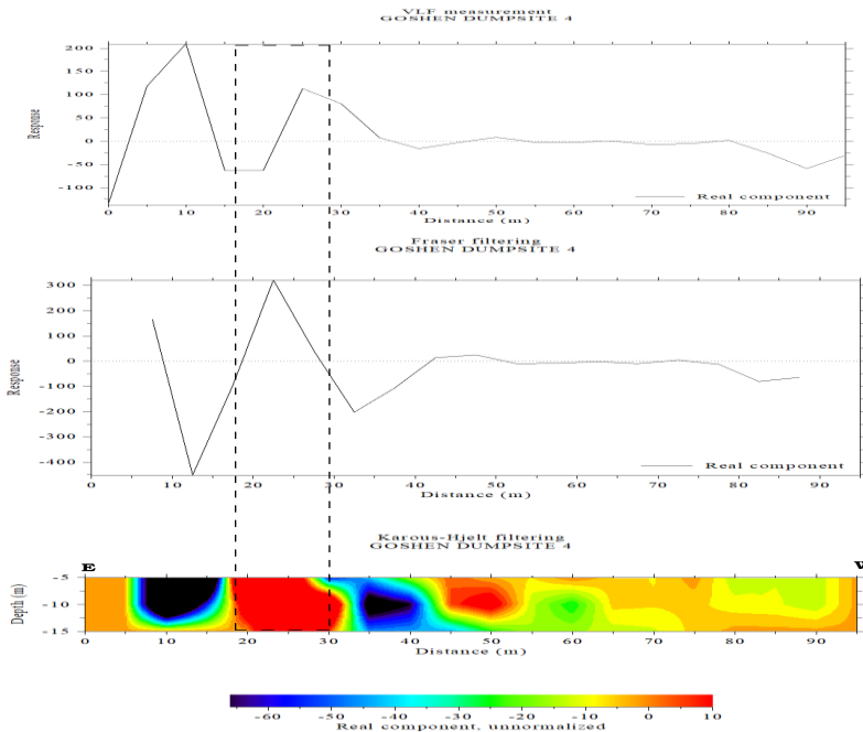
Fig. 32. Cross-section of Fraser Filtered, measured VLF and K-H pseudo section along Transverse 4
