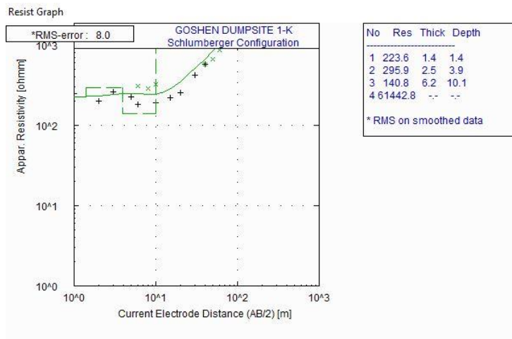
Fig. 12. Results of computer modeled curve for VES 11
