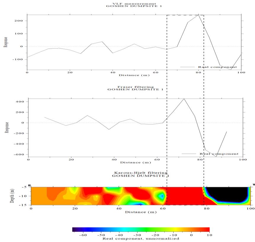
Fig. 29. Cross-section of Fraser Filtered, measured VLF and K-H pseudo section along Transverse 1
