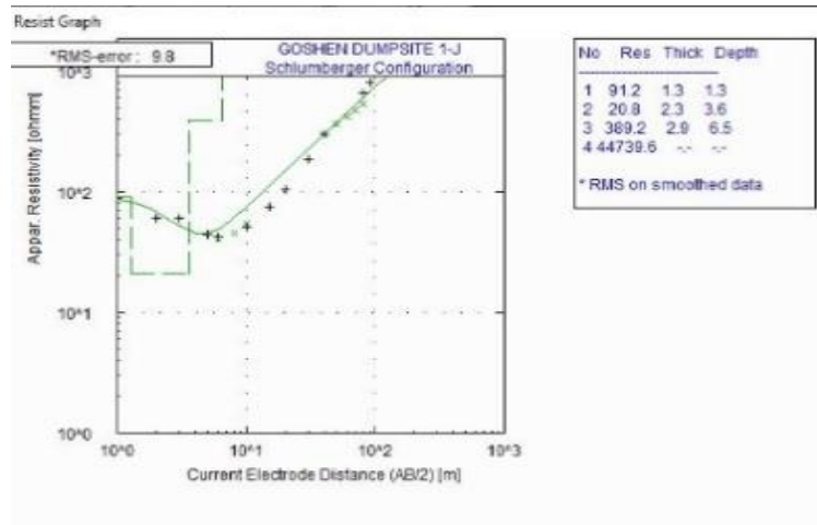
Fig. 11. Results of computer modeled curve for VES 10
