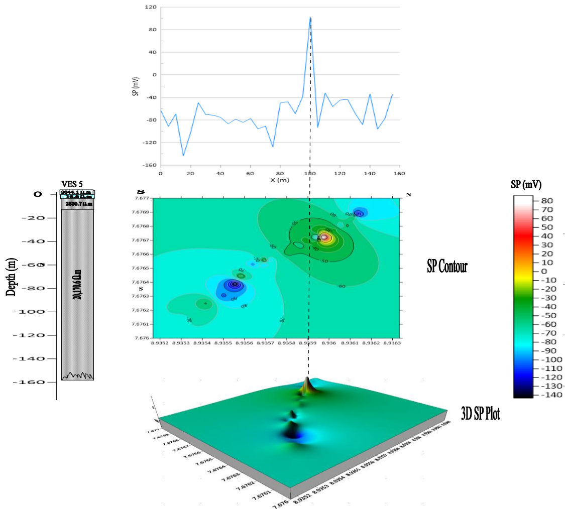
Fig. 23. Cross-section correlating the VES transverse, Self-Potential in (mV) signal, SP contours and 3-D SP plot along Profile 5
