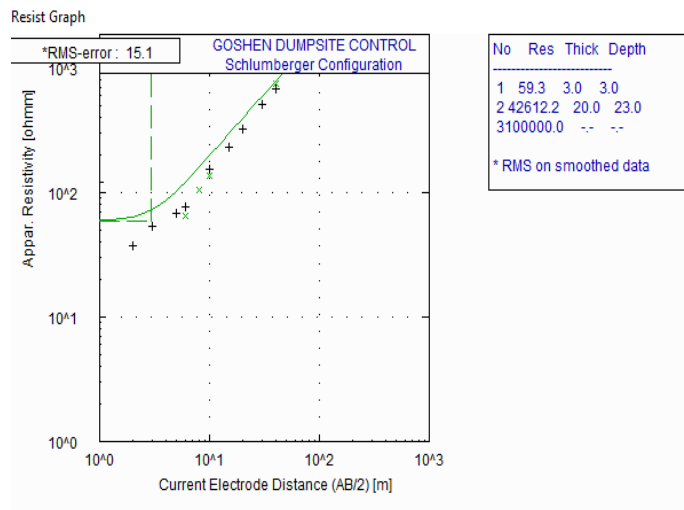
Fig. 16. Results of computer modeled curve for VES 15 (Control)
