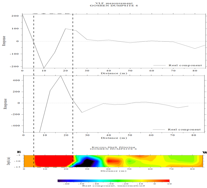
Fig. 34. Cross-section of Fraser Filtered, measured VLF and K-H pseudo section along Transverse 6
