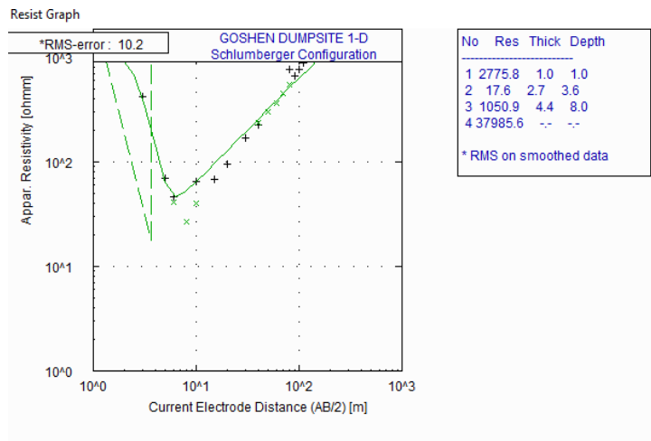
Fig. 5. Results of computer modeled curve for VES 4
