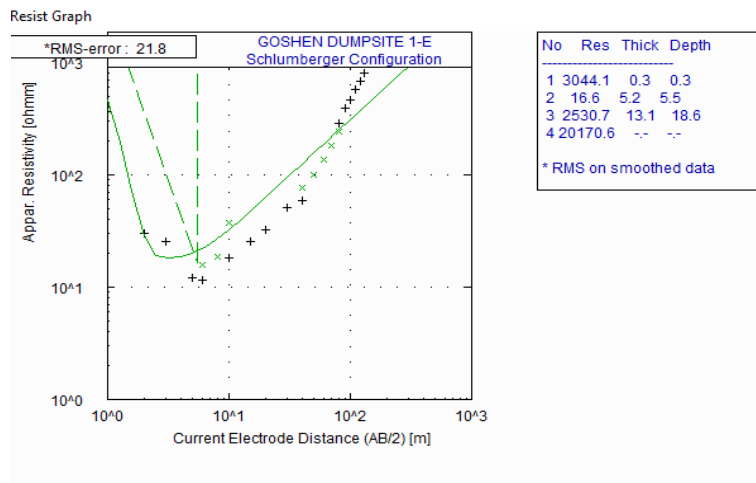
Fig. 6. Results of computer modeled curve for VES 5
