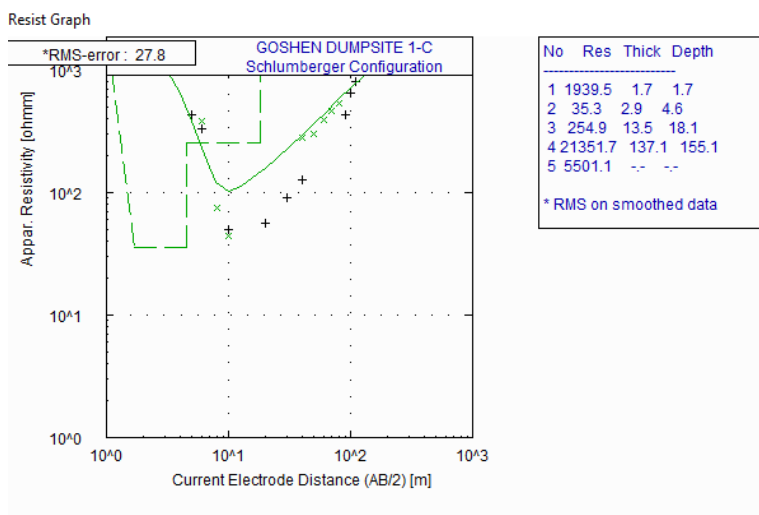
Fig. 4. Results of computer modeled curve for VES 3
