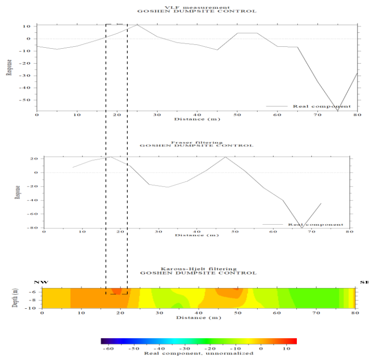
Fig. 38. Cross-section of Fraser Filtered, measured VLF and K-H pseudo section along Transverse 10 (Control Centre)
