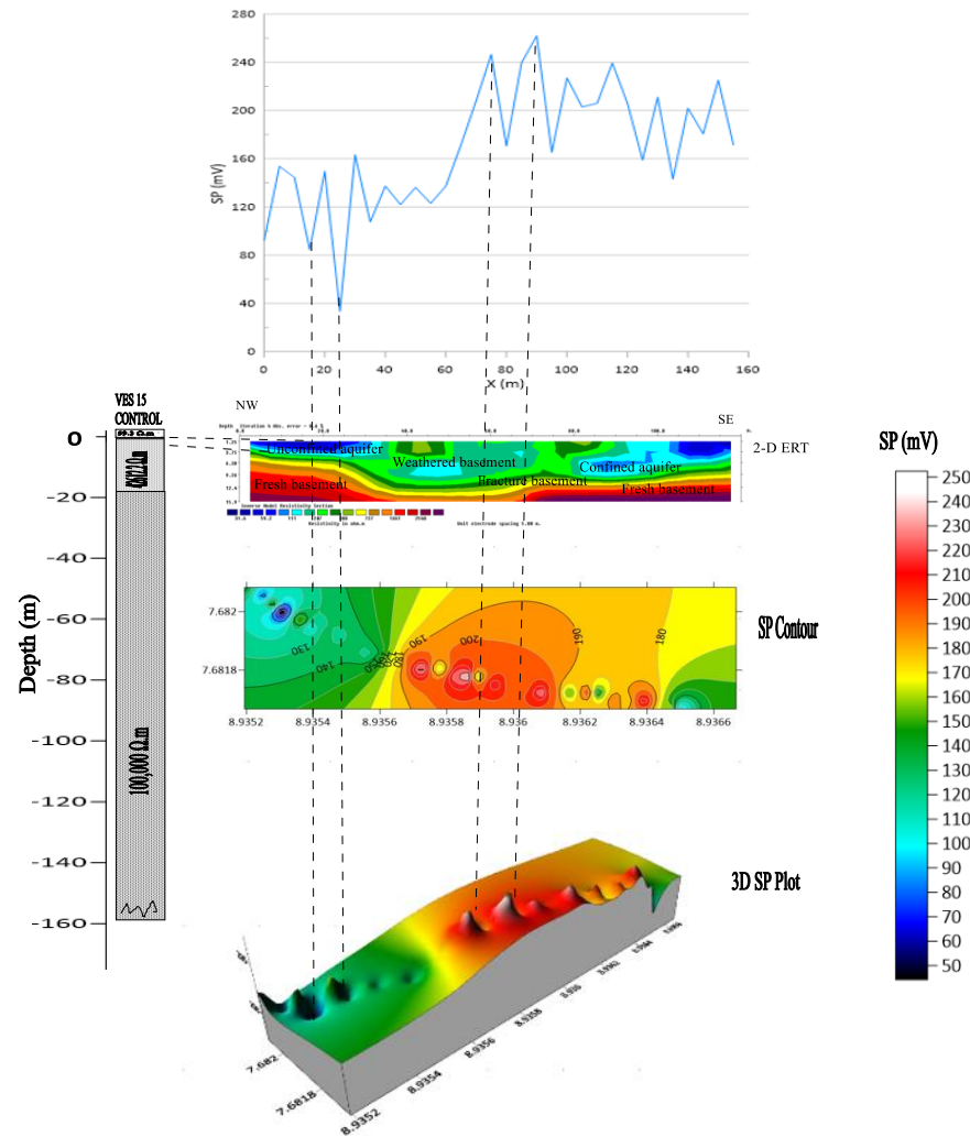
Fig. 28. Cross-section correlating the VES transverse, Self-Potential in (mV) signal, SP contours and 3-D SP plot along the Goshen Control Centre
