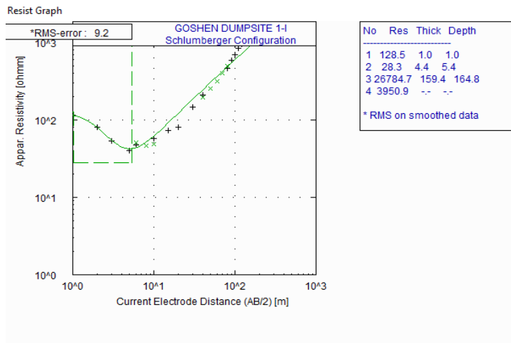
Fig. 10. Results of computer modeled curve for VES 9
