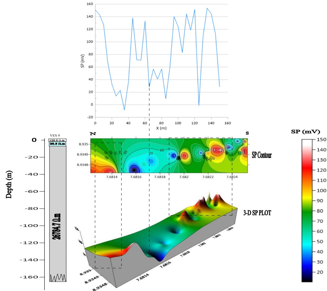
Fig. 27. Cross-section correlating the VES transverse, Self-Potential in (mV) signal, SP contours and 3-D SP plot along Profile 9 (Goshen)
