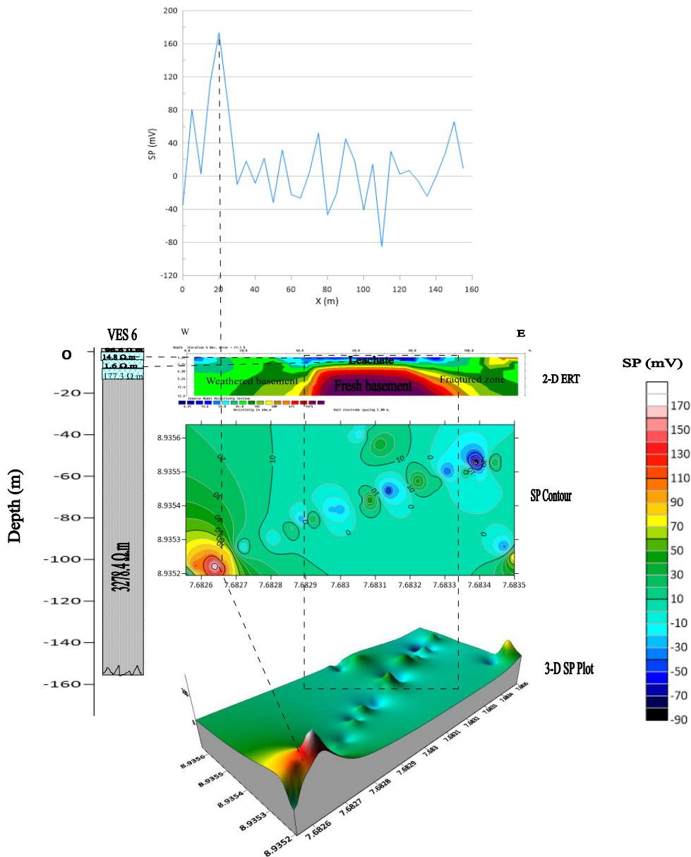
Fig. 24. Cross-section correlating the SP profile, 2-D ERT section, VES transverse, SP contour and 3-D SP plot along Profile 6
