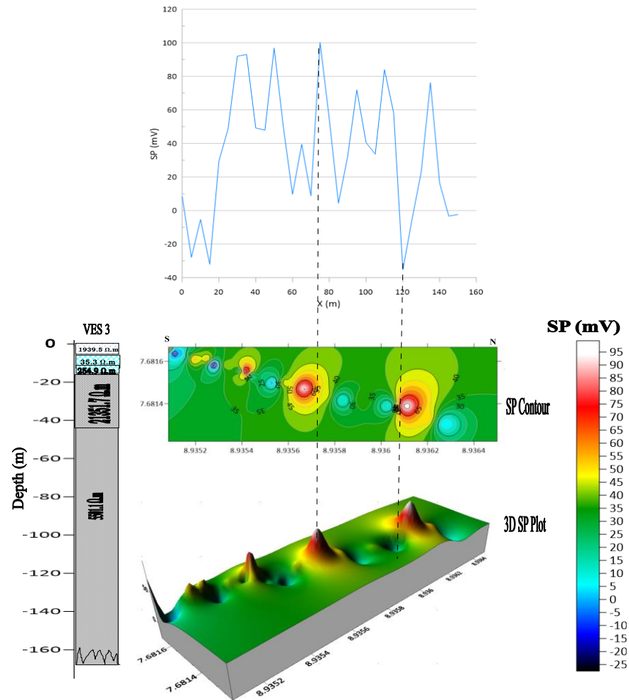
Fig. 21. Cross-section correlating the VES transverse, Self-Potential in (mV) signal, SP contours and 3-D SP plot along Profile 3
