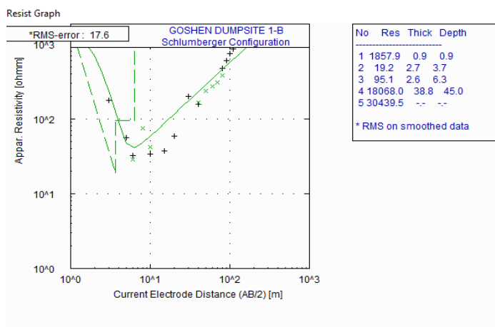
Fig. 3. Results of computer modeled curve for VES 2
