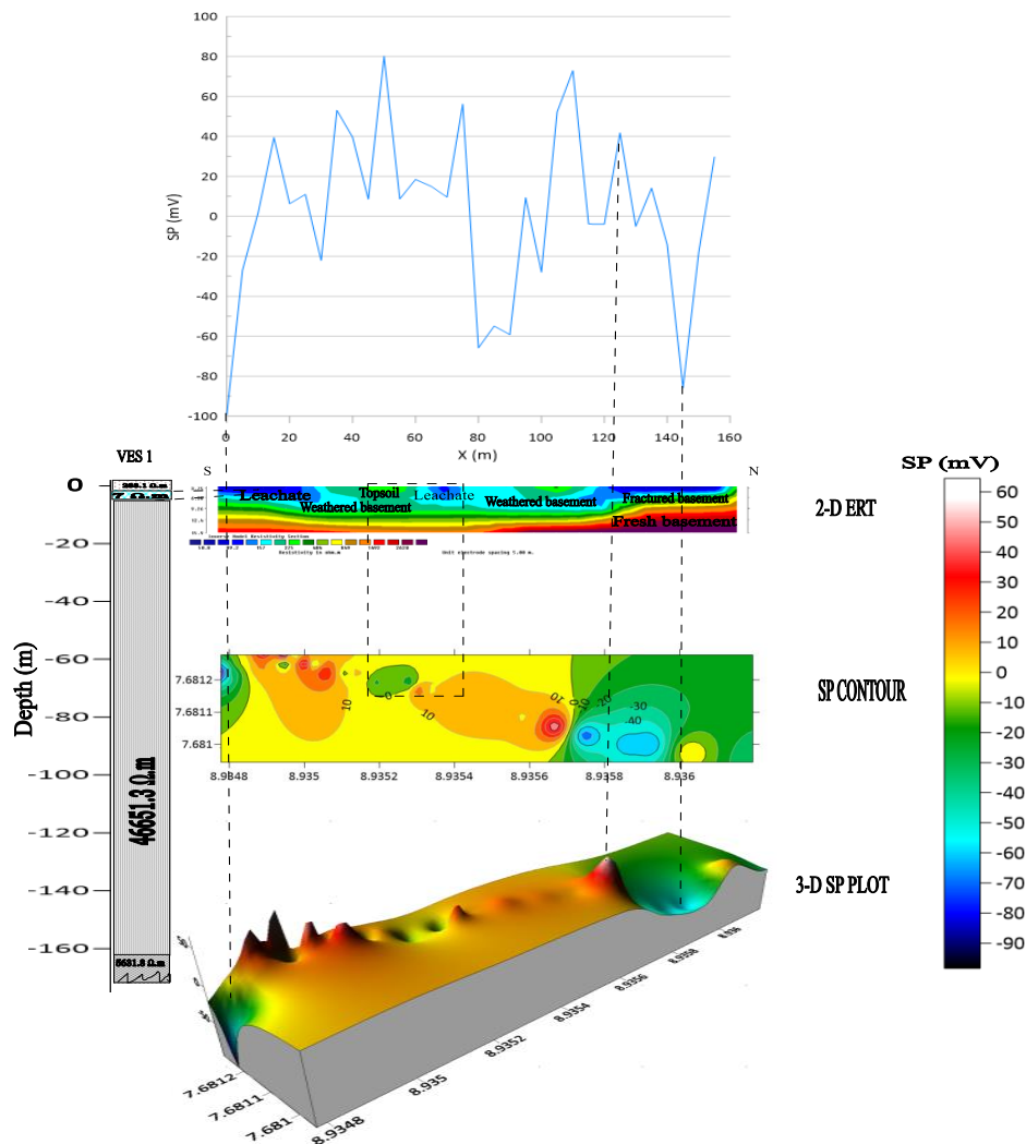
Fig. 19. Cross-section correlating the 2-D ERT geo-electric section, VES transverse, Self-Potential in (mV) signal, SP contour and 3-D SP plot along profile 1
