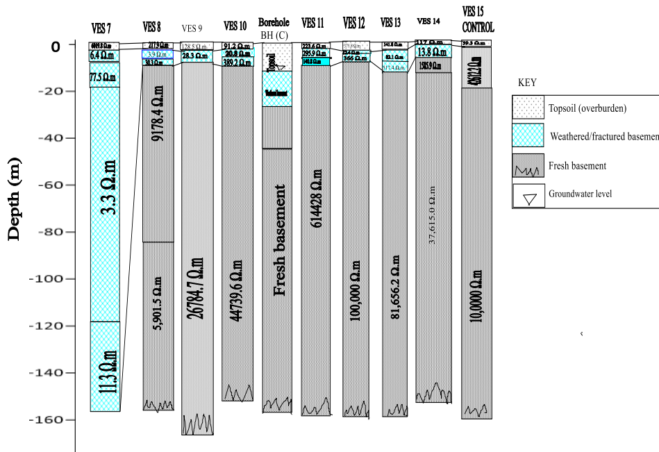
Fig. 18. Correlation of resistivity sounding (VES) results with borehole lithological logs in the study area
