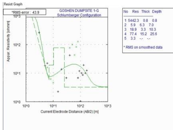
Fig. 8. Results of computer modeled curve for VES 7
