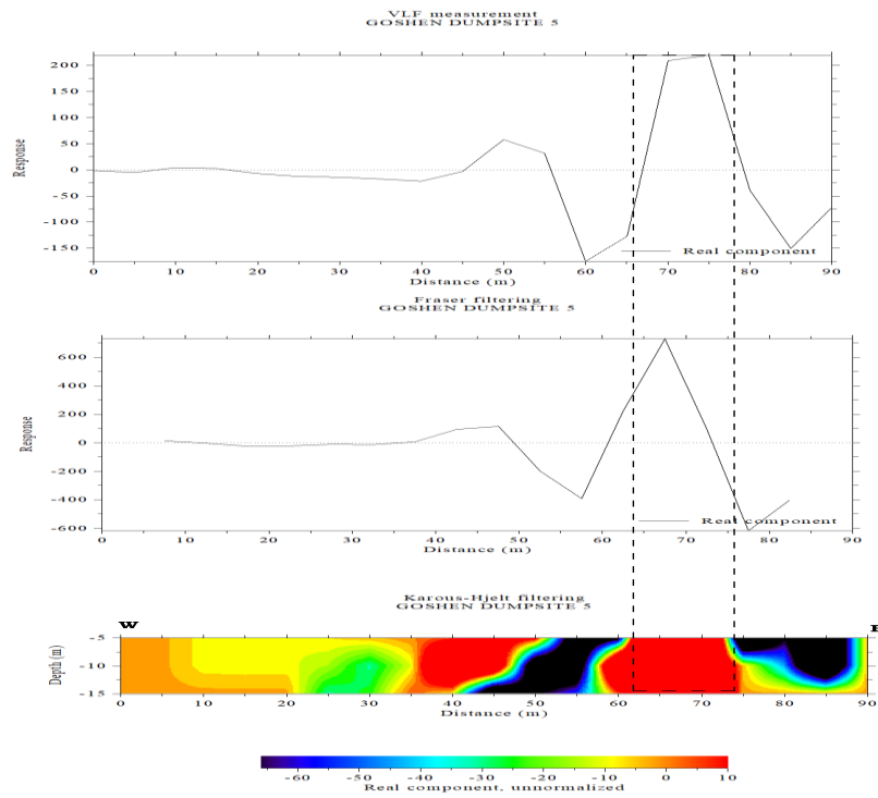
Fig. 33. Cross-section of Fraser Filtered, measured VLF and K-H pseudo section along Transverse 5
