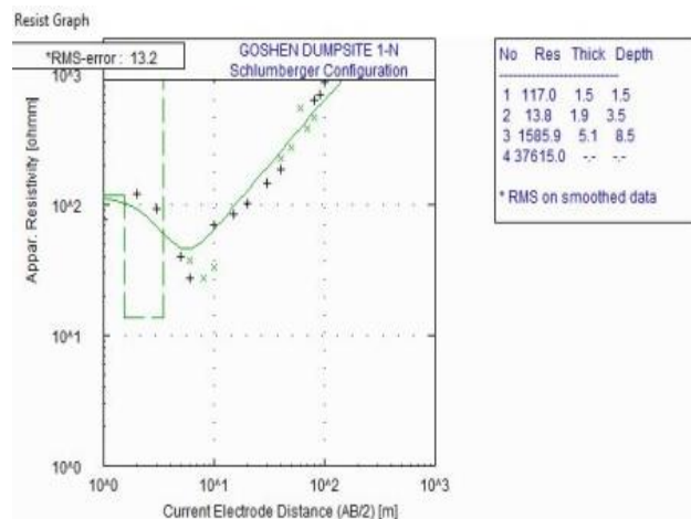
Fig. 14. Results of computer modeled curve for VES 13
