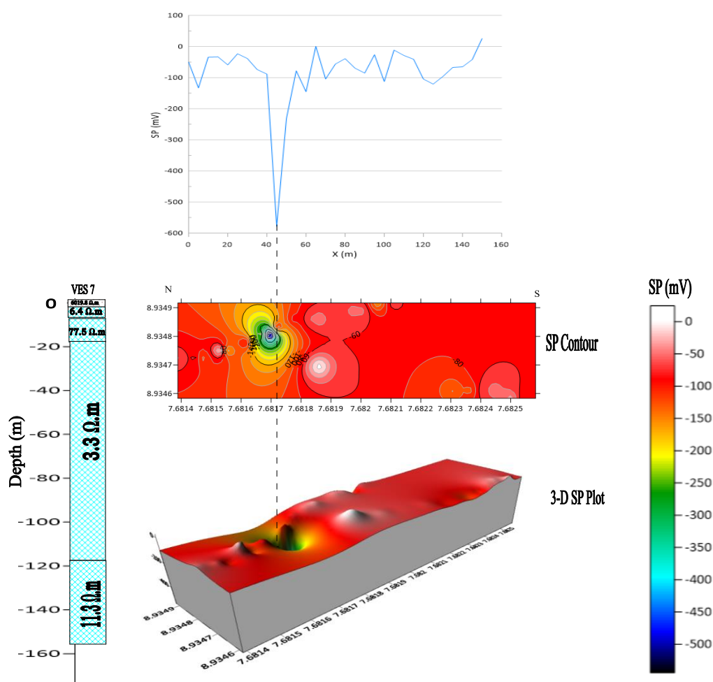
Fig. 25. Cross-section correlating the VES transverse, Self-Potential in (mV) signal, SP contours and 3-D SP plot along Profile 7
