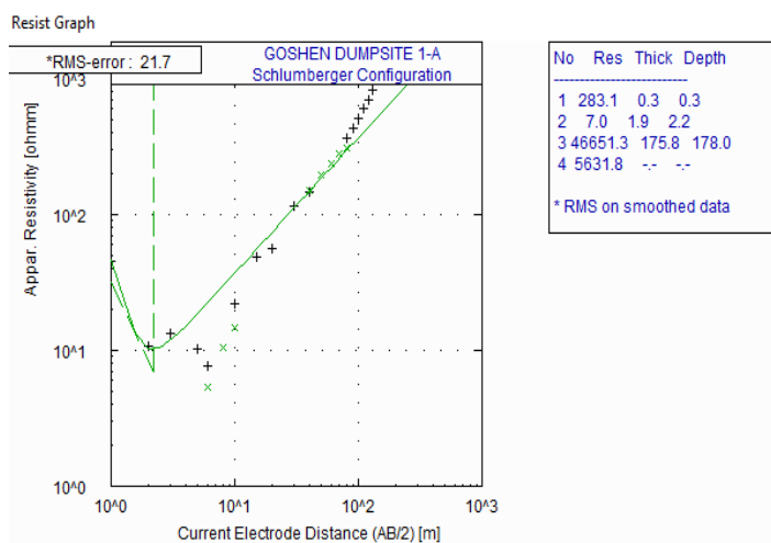
Fig. 2. Results of computer modeled curve for VES 1
