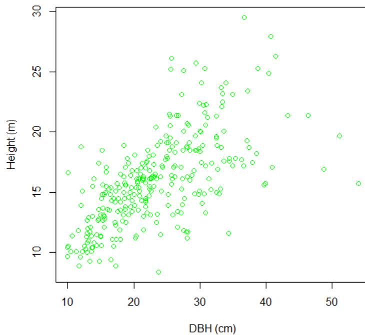
Fig. 1. Scatter plot of total height against diameter at breast height (DBH)
