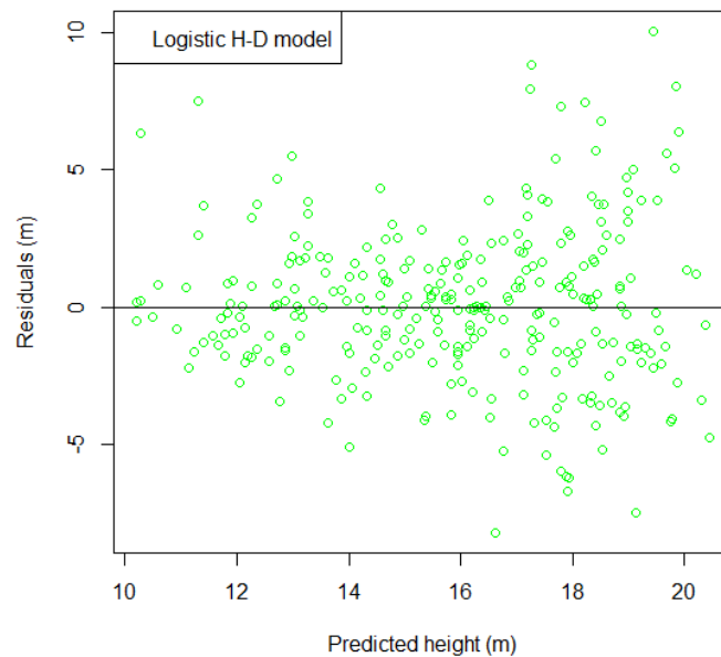
Fig. 2. Residual of the selected height-diameter model
