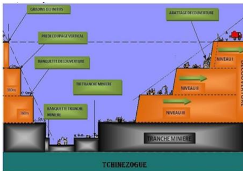
Fig. 2. Schematic cross-section of mining at SOMAÏR [16]
