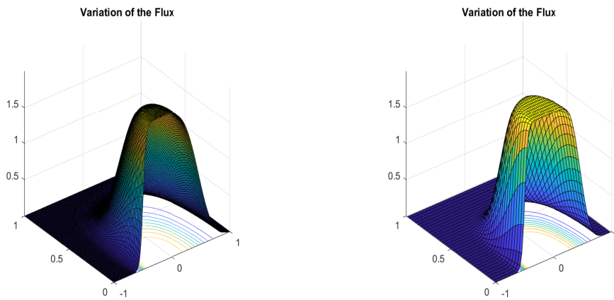
Fig. 1. Time evolution of the numerical solution
