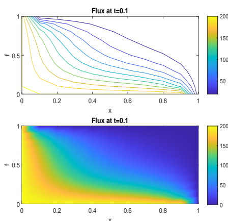
Fig. 3. Flux behavior
