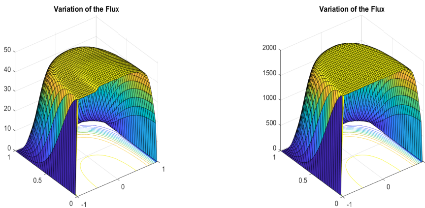
Fig. 2. Schrödinger's equation solution at various times
